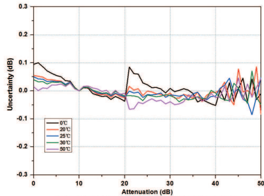
Measure attenuation switching uncertainty VS temperature of RSA3015N/RSA3030-TG/RSA3030N/RSA3045-TG/RSA3045N
