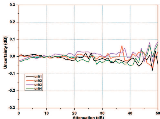
Measured attenuation switching uncertainty of RSA3015N/RSA3030-TG/RSA3030N/RSA3045-TG/RSA3045N
