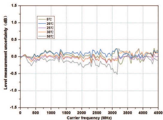
Measured level measurement uncertainty VS temperature @ -10 dBm of RSA3015N/RSA3030-TG/RSA3030N/RSA3045-TG/RSA3045N
